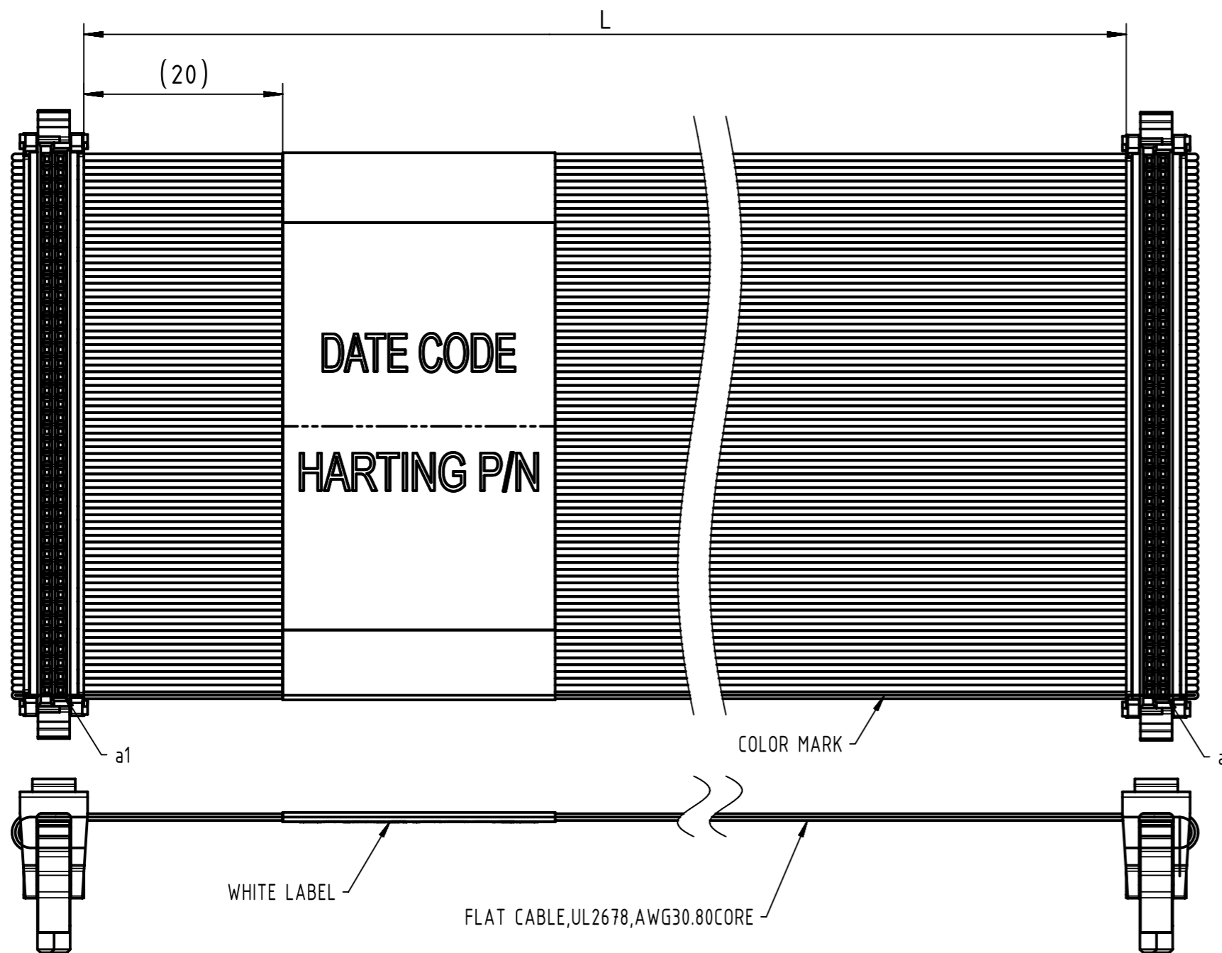
C1 HAR-FLEX 80 POLE FEMALE CONNECTOR WITH STRAIN RELIEF
