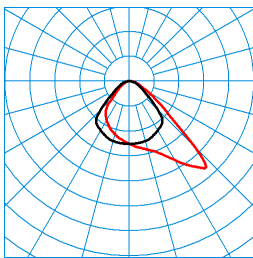
Bicult Act T G2 SMC TGCS 55 ETDI QI 01EU (ACTDCW) TX369938 ■ C0 - C180 ■ C90 - C270 DIN 5040: A50 UTE: 1,00 D CEN Flux Code: 59 89 98 100 100 0 0 0 0
