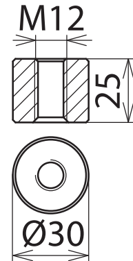
Maßbild AS SCHW M12
