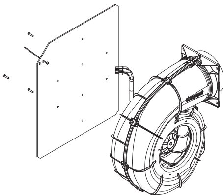
Abb. 11.2: Lüfter links
