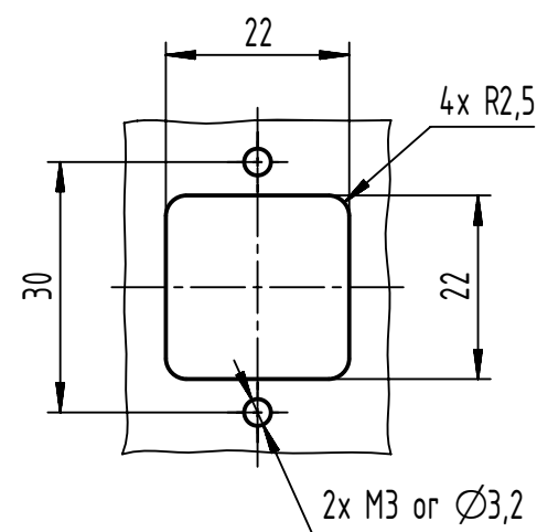
Panel cut out (1:1)
