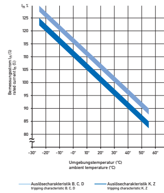
Diagramm Derating
