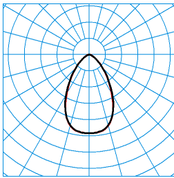
Mirona Fit BS TB 26000-840 ETDD+LLWRM IS TX197580
