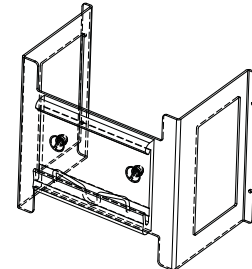
3-D-Ansicht
