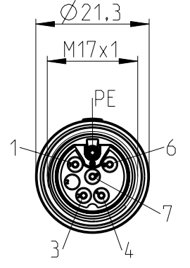
socket face female
