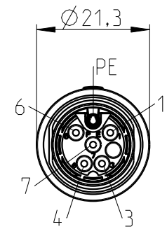
plug face male
