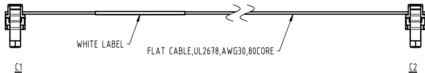
HAR-FLEX 80 POLE FEMALE CONNECTOR
