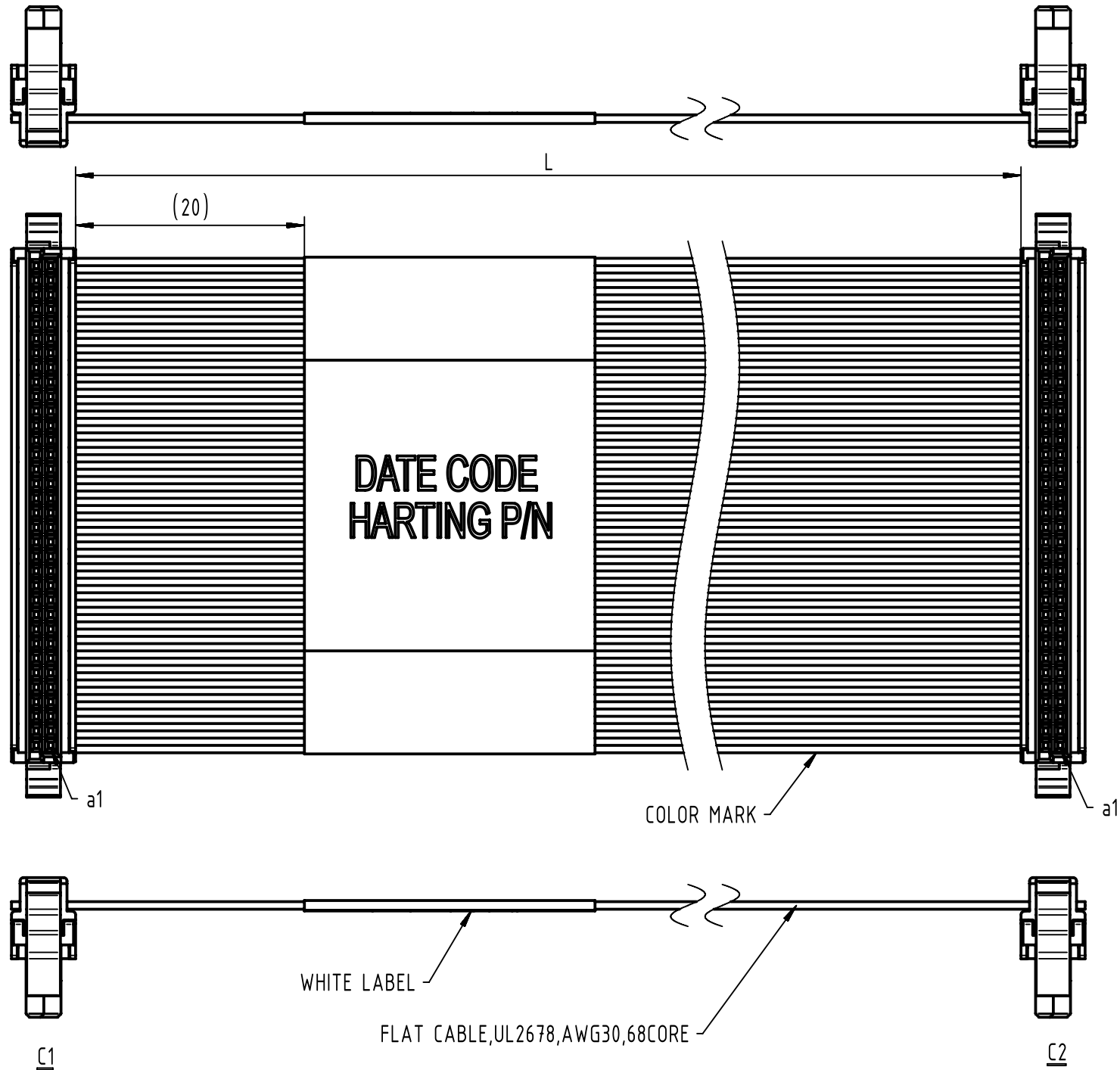
HAR-FLEX 68 POLE FEMALE CONNECTOR
