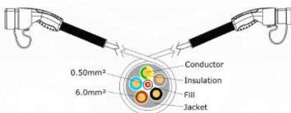
Type 2 cable
