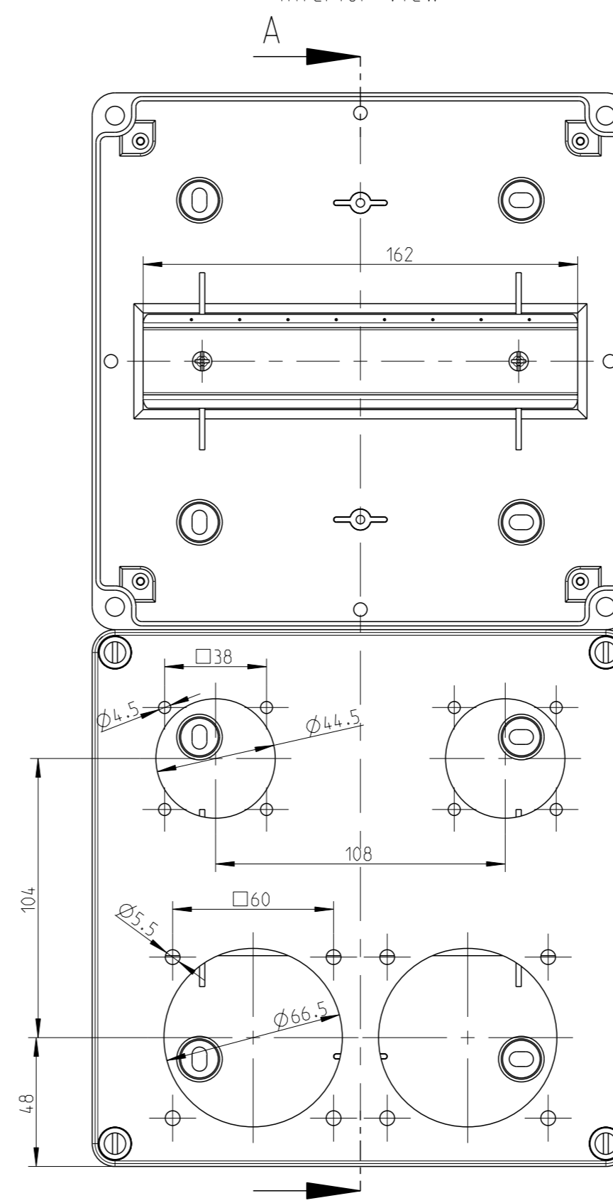
STV 922-L Innenansicht interior view
