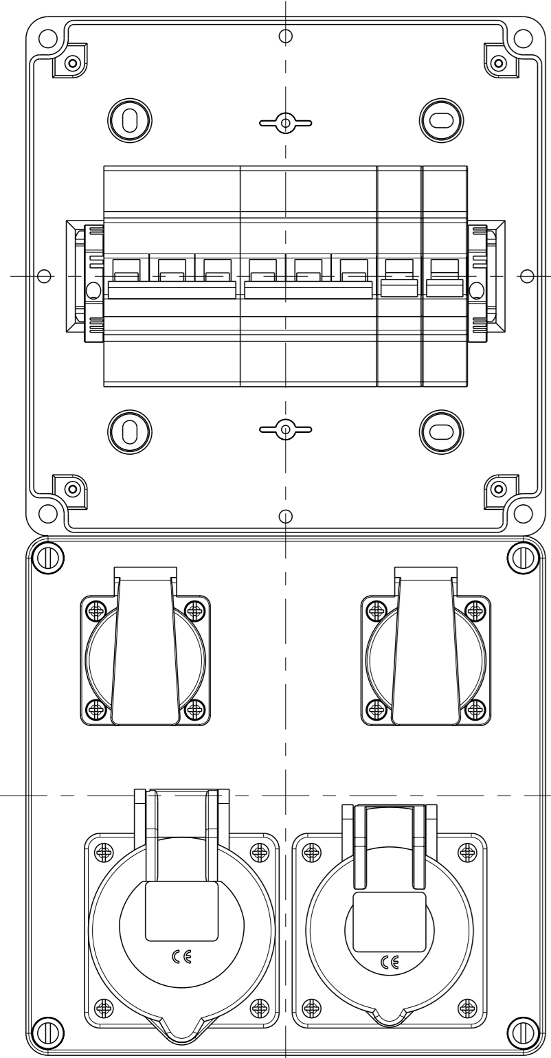
STV 922-K Innenansicht interior view
