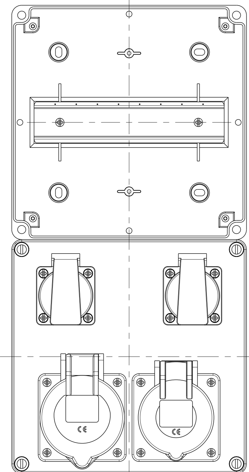
STV 922-S Innenansicht interior view
