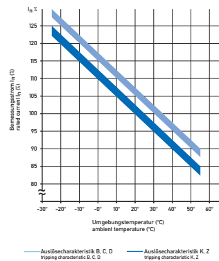
Diagramm Derating
