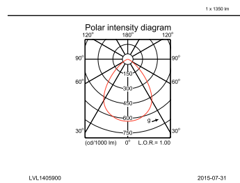
IFPC1_DN570B PSE-E 1xLED12S840 C.EPS
