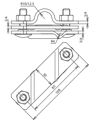
Maßbild AS S TE 20 7.10 FL40 STTZN
