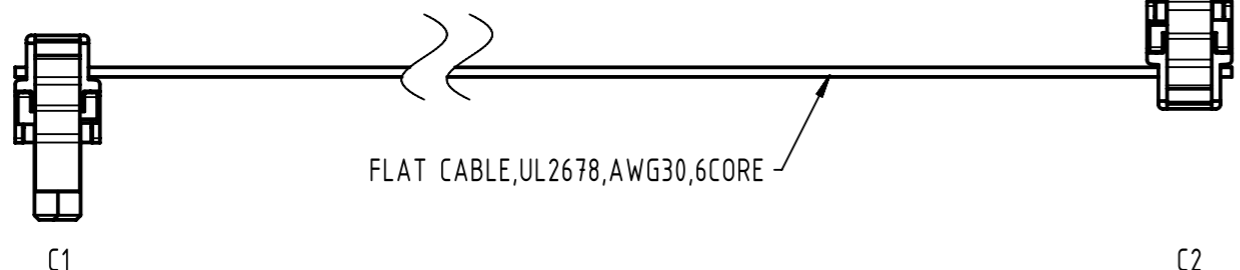
HAR-FLEX 6P FEMALE IDC CONNECTOR
