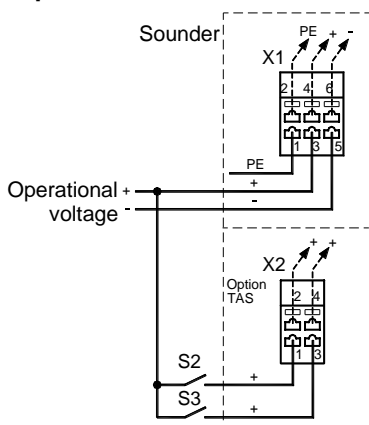
Fig. 11 Optional connection assignment TAS
