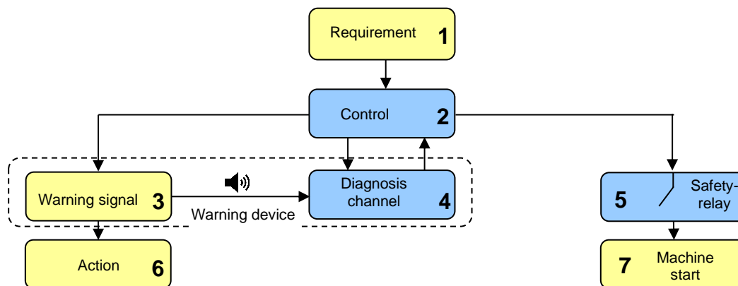
Fig. 5 Starting alarm
