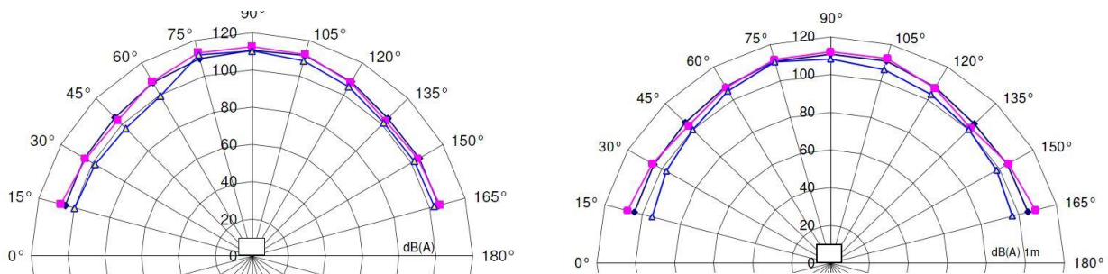
DS 10 sound pressure level horizontal diagram
