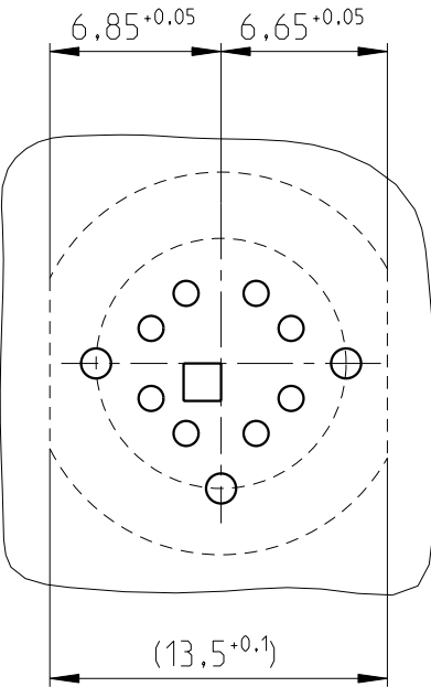
Position PCB-layout to cutout device
