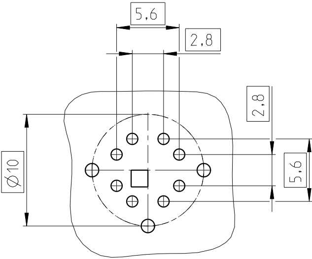
PCB-layout (advice)
