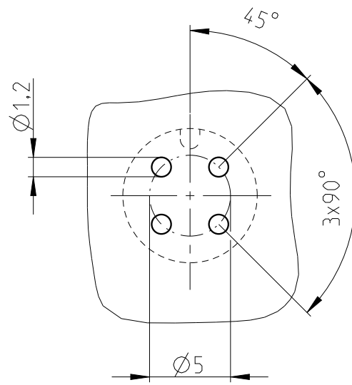
PCB-layout (advice)
