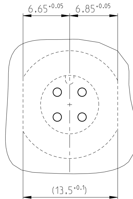
position PCB-layout to cutout device
