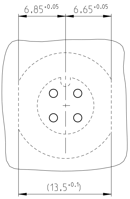
position PCB-layout to cutout device
