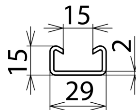
Maßbild AS SAK 1000 V2A
