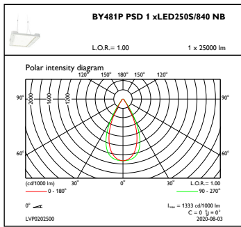
OFPC1_BY481PPSD1xLED250S840NB
