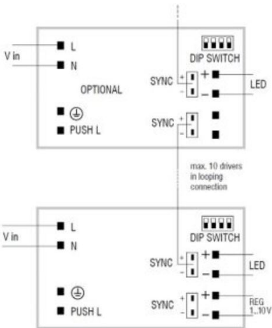
Anschlusschema 1...10 V / Potentiometer (AC/DC) Connection diagram 1...10 V or potentiometer (AC/DC)
