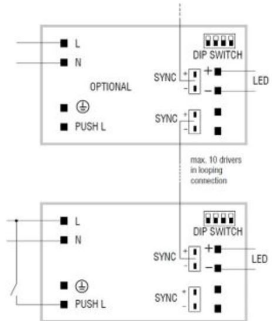
Anschlusschema Push button (AC) Connection diagram with push button (AC)
