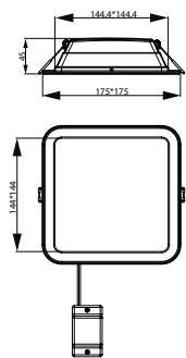
DN065B G4 LED12/830 12W 220-240V L150 SQ
