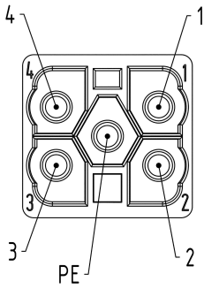
Mating face
