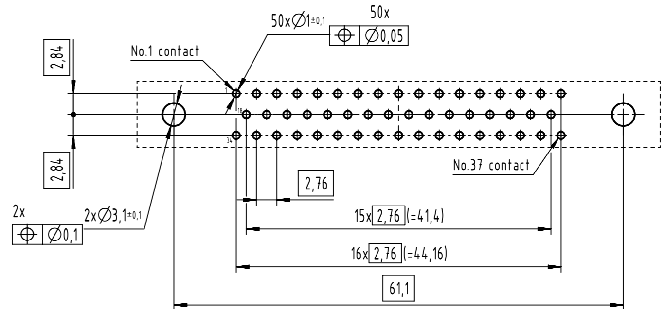
PCB layout hole component side
