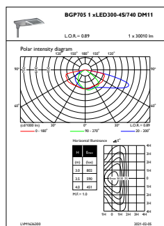
OFPL1_BGP7051xLED300-4S740DM11
