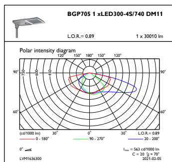
OFPC1_BGP7051xLED300-4S740DM11
