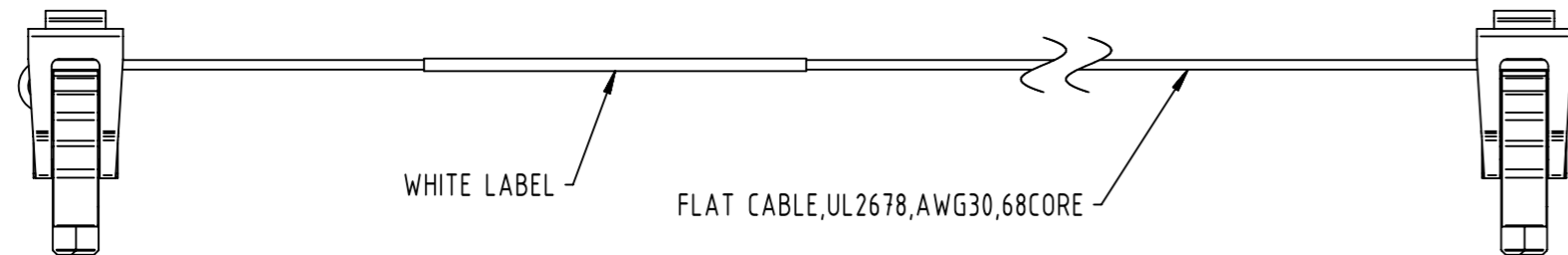
C1 HAR-FLEX 68 POLE FEMALE CONNECTOR WITH STRAIN RELIEF
