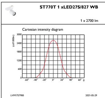
IFCC1_ST770T1xLED27S827WB
