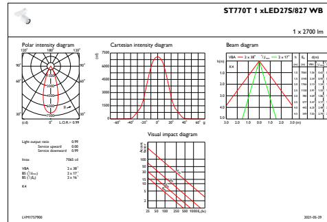
IFAS1_ST770T1xLED27S827WB
